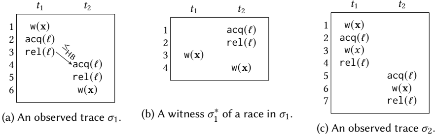
Fig. 1. (1a) shows a trace \sigma_1 with a sync-preserving race ( e_1, e_6 ) missed by \leq_{\text{HB}} . (1b) shows a witness that exposes the race. (1c) shows a sync-preserving race ( e_1, e_6 ) that is non-consecutive, due to the intermediate event e_3 .
