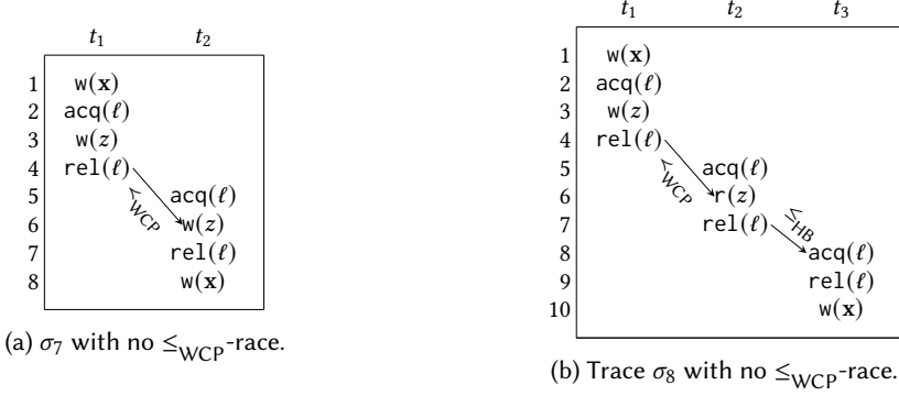
Fig. 7. Traces \sigma_7 and \sigma_8 have sync-preserving races. But \leq_{\text{WCP}} does not report any races.
