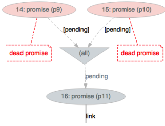
Fig. 8. Example of unsettled promise, Actions on Google.
