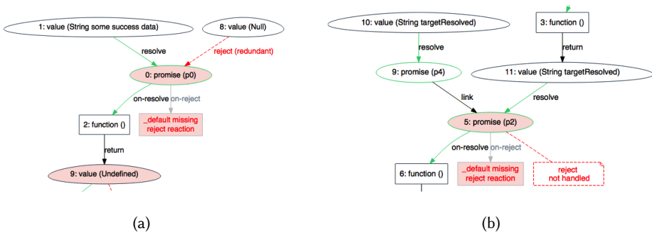
Fig. 11. Examples of multiple settle, Razorpay (11a), and unnecessary promise, Promise Branch (11b).
