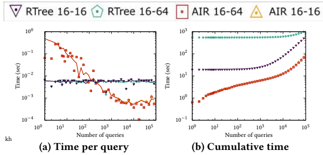
Figure 16: Uniform 2D shape data & workload, R-tree forms.
