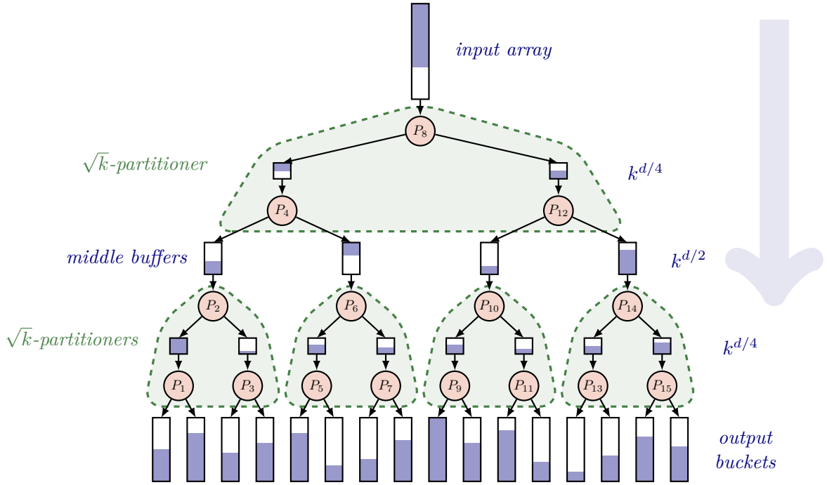
■ Figure 2 A k -partitioner for k = 16 buckets. Content in the buffers is shaded; buffers are filled bottom-to-top; when full, they are flushed and then consumed from the bottom. The figure shows the situation where the input buffer for P_6 is being flushed down to its children (by partitioning elements around pivot P_6 ). The flush at P_6 was triggered during flushing P_4 's input buffer, which in turn has been called while flushing P_8 (the input).
