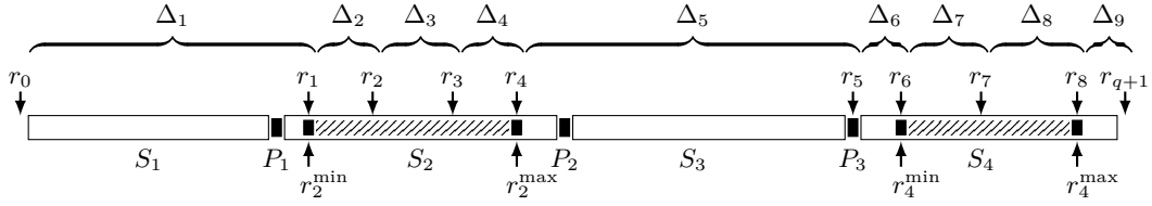
■ Figure 3 Deterministic multiple selection. The partition of an array S into buckets S_1, \dots, S_4 separated by pivots P_1, \dots, P_3 , and query ranks r_1, \dots, r_8 . In the example the maximum allowed bucket size is \Delta = \Delta_1 , since \Delta_1 + \Delta_2 + \Delta_3 + \Delta_4 + \Delta_6 + \Delta_7 + \Delta_8 + \Delta_9 \geq |S|/2 + 1 and \Delta_2 + \Delta_3 + \Delta_4 + \Delta_6 + \Delta_7 + \Delta_8 + \Delta_9 < |S|/2 + 1 . Black squares are pivots and the shaded regions in buckets are the subproblems to recurse on.
