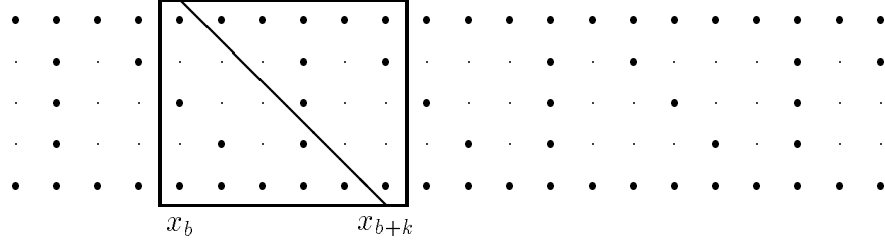
Figure 2: The division of a block of the computation graph in Figure 1 into “triangles”.
