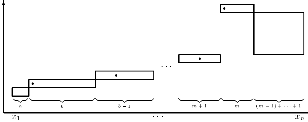
Figure 5: The ordering of elements for the augmented staircase problem. The black points indicate the x_{c_i} 's.
