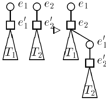
Figure 4: The first step of a MELD operation (the case e_1 \leq e_2 < e'_1 \leq e'_2 ).
