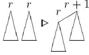
Figure 3: The linking of two nodes of equal rank.
