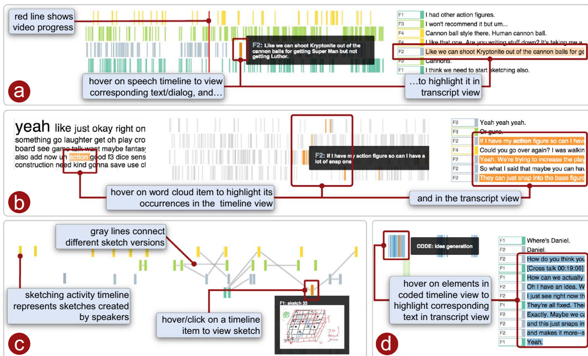
Fig. 4. Various forms of brushing and linking used in the framework, to facilitate the envisioned orient and focus tasks. (a) shows the transcript text on the right, linked to a time-sequence representation of utterance “events” color-coded by speaker ID. Hovering on an element in the time-sequence view highlights the corresponding text in the transcript view, and vice versa. (b) shows similar interactive linking, but this time, hovering on a word in the word cloud shows all its occurrences in the time-sequence and text views. (c) shows the sketch log view, where each “event” represents a sketch save operation. A hover event on this view shows a thumbnail of the saved sketch. The interactions in (d) are similar to (a) except the time-sequence view shows all utterance events assigned to a particular user-defined code.
