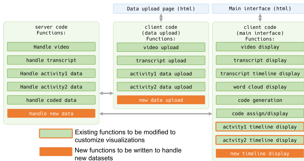
Fig. 8. An overview of the high-level functions in VizScribe, showing the functions that need to be modified in order to edit or customize existing timeline visualizations, and functions that need to be added in order to create new timeline visualizations. Fig. 9 shows conceptually how these visualizations can be customized. Templates for functions are also available in the VizScribe source code page (see footnote 8) with detailed instructions on its Wiki.
