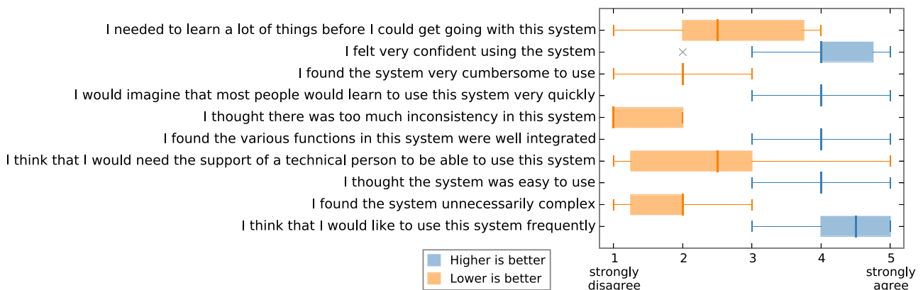
Fig. 12. The System Usability Study (SUS) scores shown category-wise, aggregated over all participants. Plots in orange are better when lower, while plots in blue are better when higher. An mean rating of 75.5/100 was obtained.
