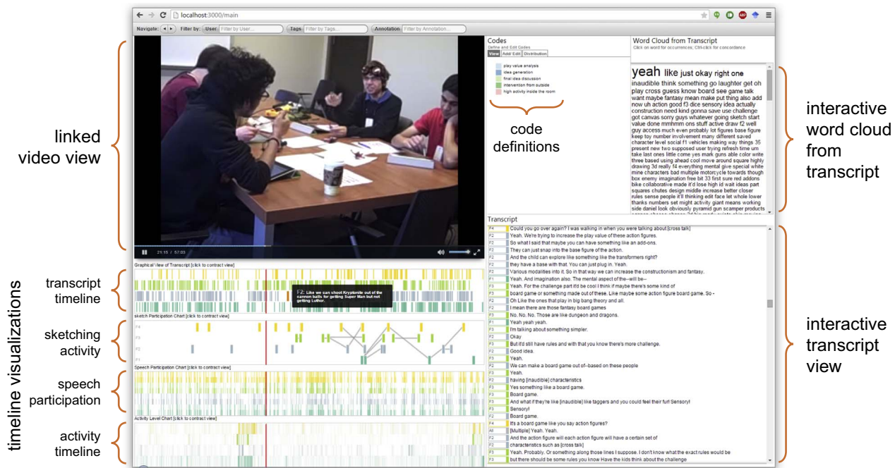
Fig. 1. A screenshot of VizScribe shows representations of video, transcript, sketching activity, speech participation, and physical activity based on corresponding data. These data are displayed as interactive timeline views, such as video progress, transcript visualization, and sketch timeline. Word cloud and transcript views also allow the user to interact directly with the data. The user can jump to a specific part of the video by clicking the transcript, and can select a line to assign it a specific code. A short demonstration of VizScribe can be seen here: https://vimeo.com/169905057 .
