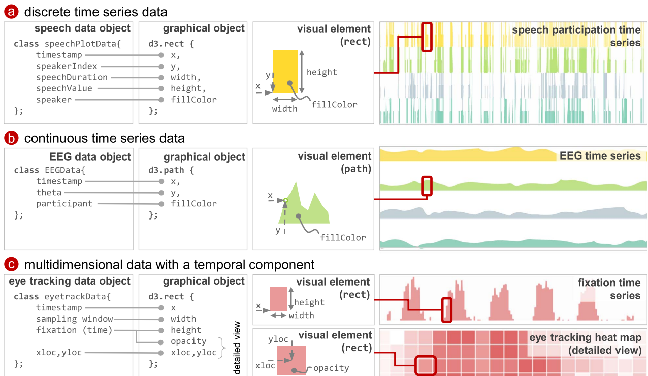
Fig. 9. Extending or customizing a timeline visualization to fit custom time-series data involves mapping attributes of that data to a corresponding visual object. VizScribe uses D3 for this purpose, whose data structure makes this mapping possible. The above figure illustrates how this extension is possible for three main categories of data, namely a discrete time series data where data is sampled at intervals, b continuous time series data where data is read in a stream, and c multidimensional data with a temporal component, where a time series visualization needs to be augmented with additional visualizations. For all three categories, the above figure illustrates ways in which the VizScribe timeline views can be extended to incorporate such data by mapping data attributes to geometric attributes of appropriately chosen D3 elements. Hover/click behaviors are then specified, allowing for interaction with the data.
