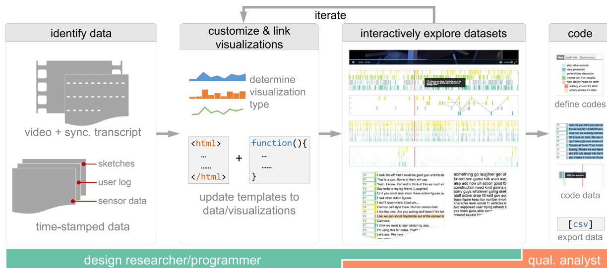
Fig. 7. Visualization pipeline used in the VizScribe framework. The standard inputs (required) are in the form of a video and a timestamped transcript. The VizScribe web application generates a default timeline and word cloud visualization for the transcript. Predefined code “templates” cater to other timestamped code, where the researcher, based on step-by-step instructions in the VizScribe Wiki, can iteratively customize these templates to explore different interactive visualization forms. Once the visualizations are finalized, the researcher can begin coding the transcript and exporting the coded data to a comma-separated value (csv) file.
