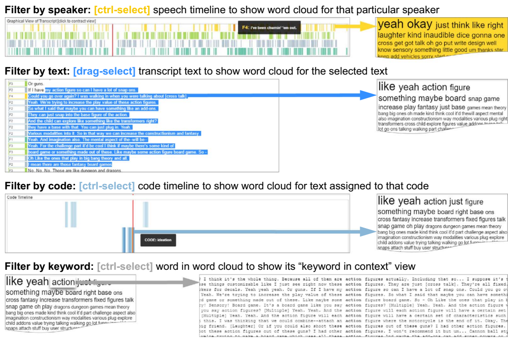
Fig. 5. Some of the filtering options available between the timeline and text views in VizScribe. The users can focus on specific parts of the datasets by filtering, say, the word cloud display by speaker or by the assigned code. They can also directly select a section of the transcript, which updates the word cloud to the selected text, providing an overview of the text. Finally, a keyword in context (KWIC) view of a word of interest provides a way to understand the context of its use in the transcript.
