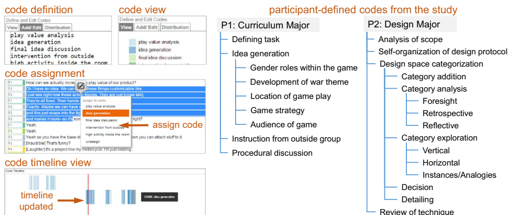
Fig. 6. Coding in VizScribe and sample codes generated by participants from our formative studies. The screen captures from VizScribe on the left show the code definition and code assignment. The hierarchical codes on the right were defined by the participants (P1 & P2) in the formative study. Though using the same dataset for the coding task, the participants produced very diverse codes, based on their research backgrounds (curriculum development vs. design).
