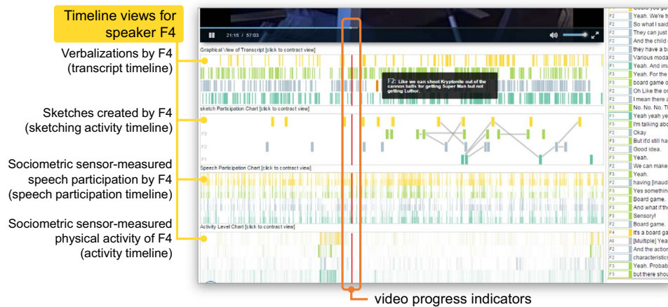
Fig. 2. Detail of VizScribe's temporal view. The video used in this example has four participants or speakers, and thus each participant's activities are color-coded and displayed on the timeline. In this figure, all activities of participant F4 are illustrated as an example. The timeline of verbalizations shows a series of markers (■) indicating instances of F4's speech. Similarly colored markers are used for the remaining timeline views for F4.
