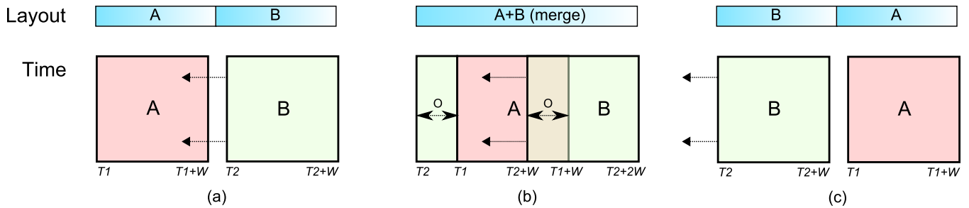
Figure 6: Layout and temporal view of merge operations for strips during temporal overlap. (a) Two strips, A and B, at time positions T_1 and T_2 , respectively, and both of interval width W are approaching. (b) Temporal overlap between A and B, causing the layouts to merge into a single strip. To maintain the same combined layout size on the visual space, all temporal overlap is added to the beginning of the combined interval. (c) B has now passed A and there is no longer a temporal overlap, so the strips are separate and with correct temporal order in layout space.
