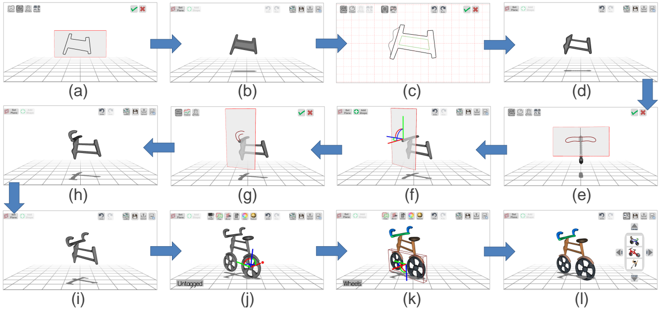
Figure 2. General 3D design workflow in Co-3deator with a bicycle design example: (a-b) Using a tapered blobby shape to define the bike frame (first shape), (c-d) Adding a hole and modifying the shape (with overdrawing) on the bike frame, (e) Setting a plane at the tip of the frame and defining the handlebar with a rounded blobby shape, (f) Setting sketch plane - manipulation widget allows users to adjust plane position, (g-h) Defining a handlebar grip using tubular shapes, (i) Mirroring the handlebar grip about the frame, (j) Completing the design by adding seat and wheels - the read wheel shapes are copied, (k) The shapes are colored/textured and tagged to an appropriate part- each part can be selected and manipulated as a single entity, (l) Design Explorer viewed in 3D workspace.
