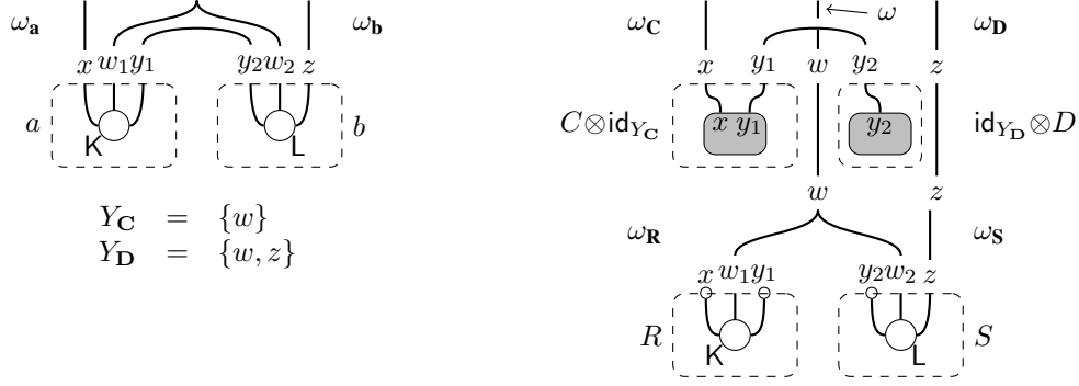
Figure 4: Matching a product using the PAR rule
