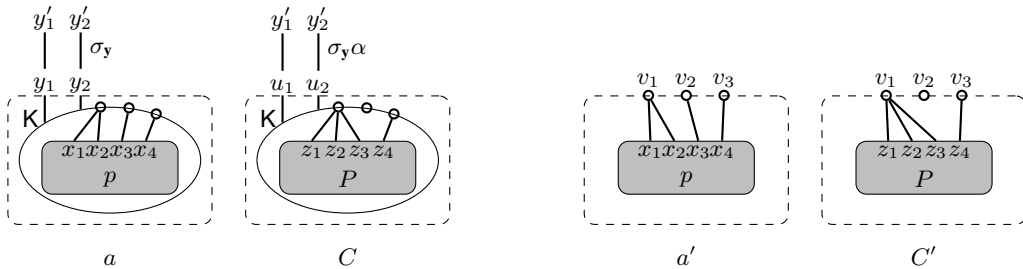
Figure 5: Matching ion agent a yielding context C by matching a' yielding context C'
