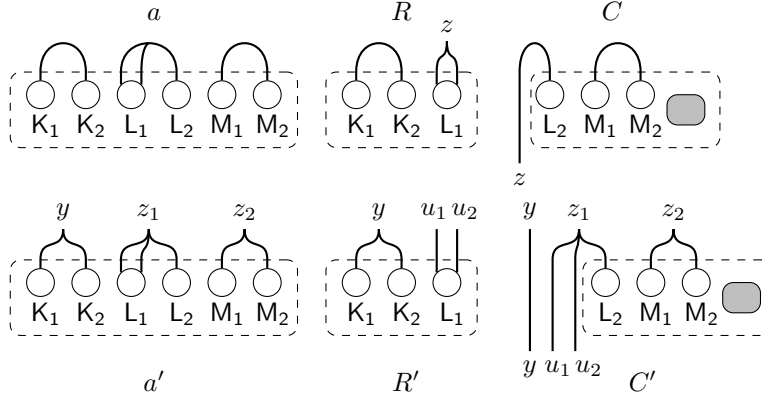
Figure 6: Matching closed links within and between redex and context
