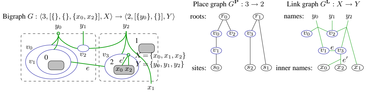
Figure 2: Example bigraph illustrated by nesting and as place and link graph.
