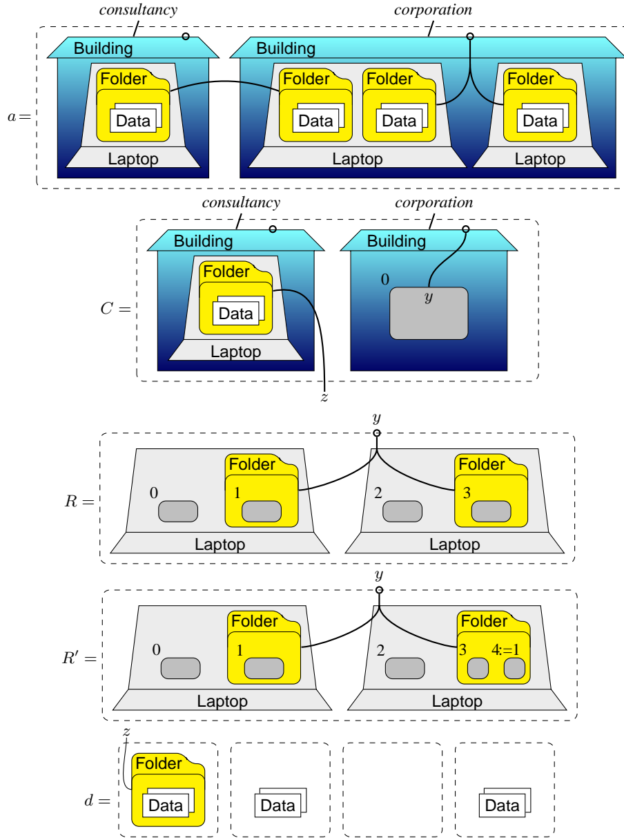
Figure 1: Example of a ground agent a = C \circ (\text{id}_z \otimes R) \circ d . Reaction rule R \rightarrow R' copies data between connected folders.
