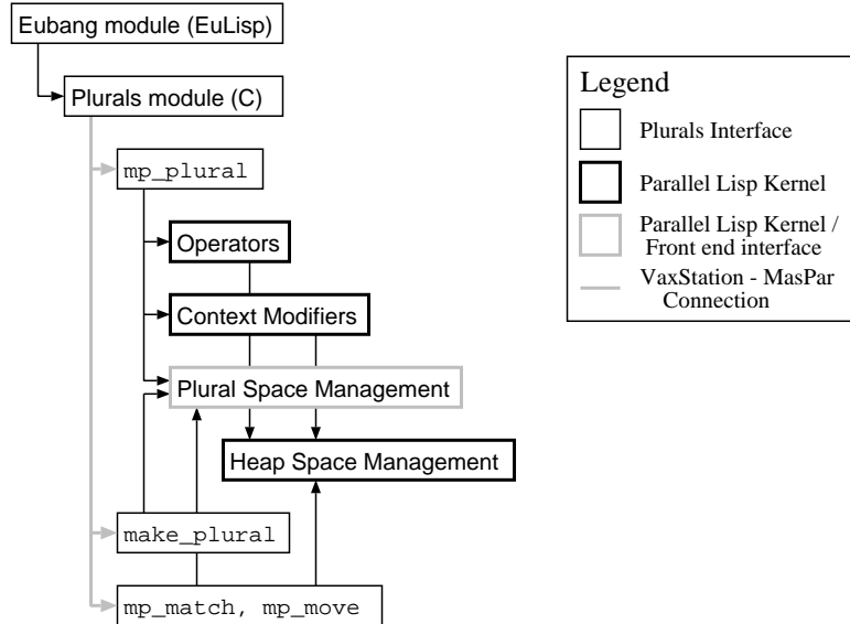
Figure 1: System Organisation
