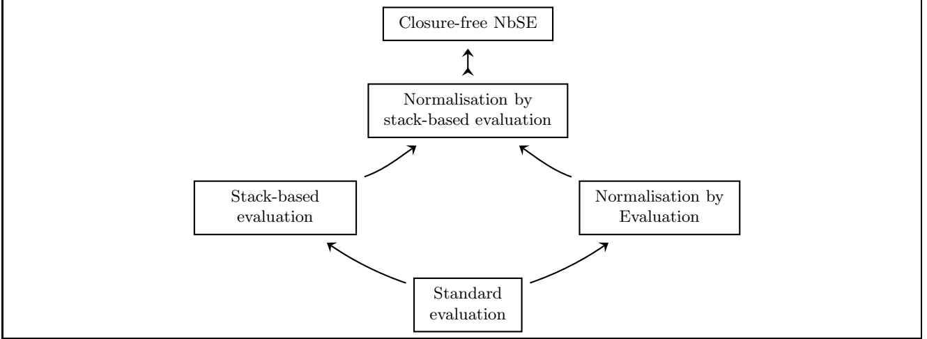
Figure 5. Normalisation by stack-based evaluation as a conservative extension, \longrightarrow , of stack-based evaluation, Normalisation by Evaluation, and standard evaluation, plus the derivation, \rightsquigarrow , of closure-free NbSE
